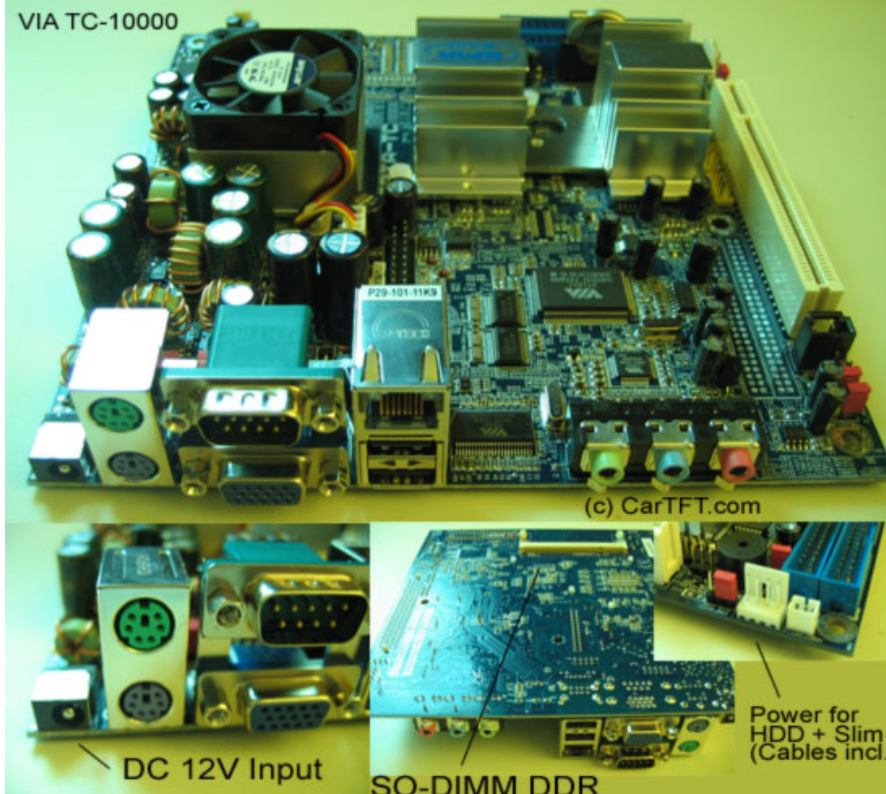
VIA EPIA TC10000
